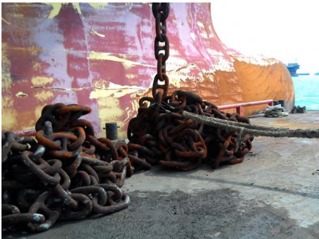
Secured anchor chain with lashing rope
