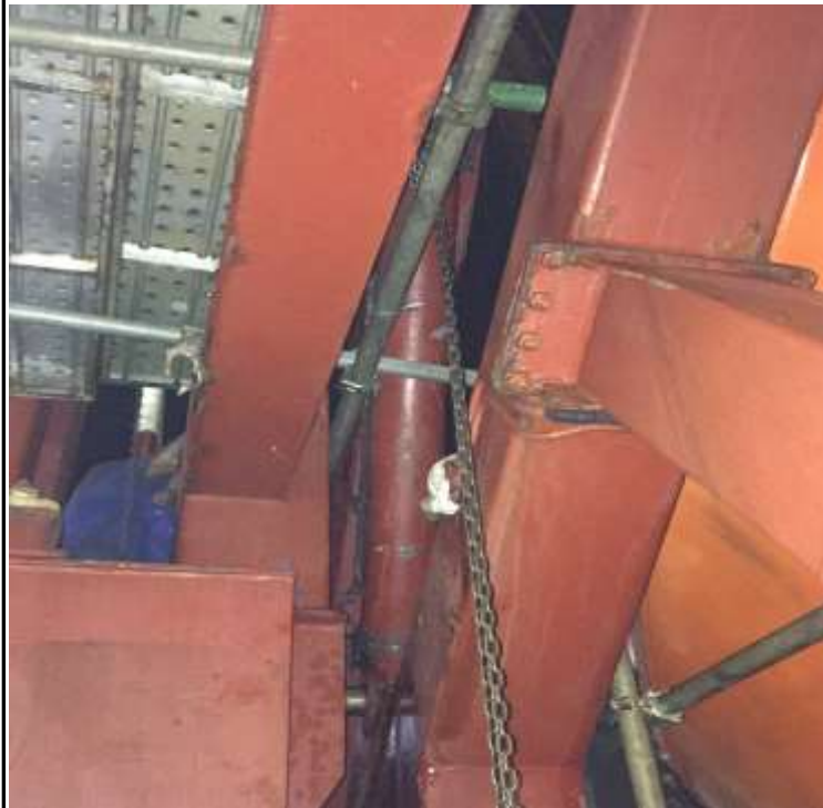
Lifting Hydraulic Cylinder manually in place after thorough cleaning of hinges
