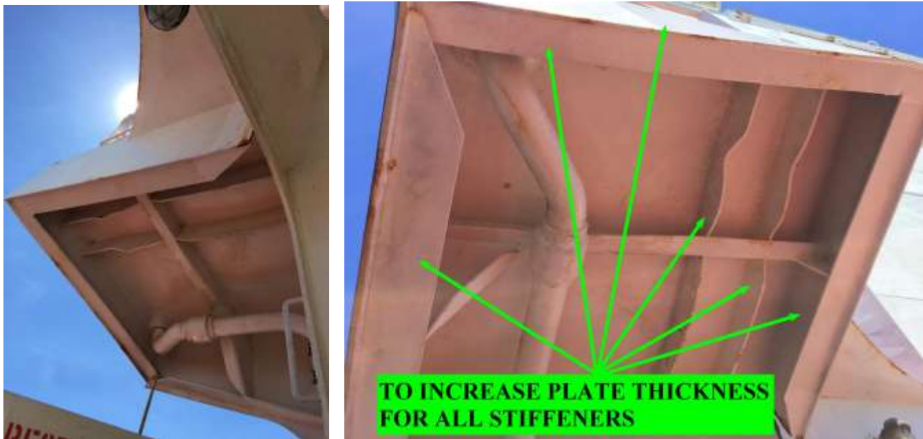
Thickness of steel material for deck structure to be increased
