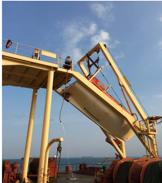
Discharging water from water bags
