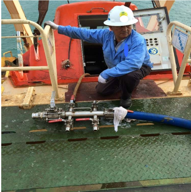
Filling water to the water bags
