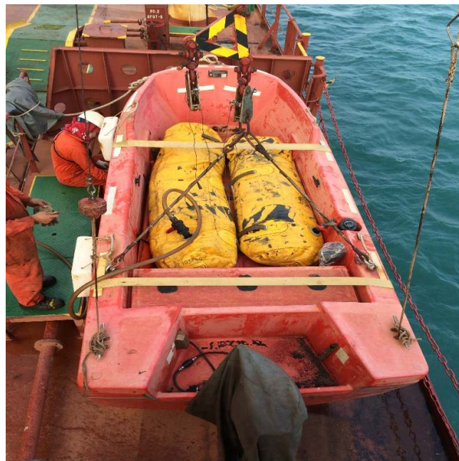
1.5 bags x 375 kgs/ bag
